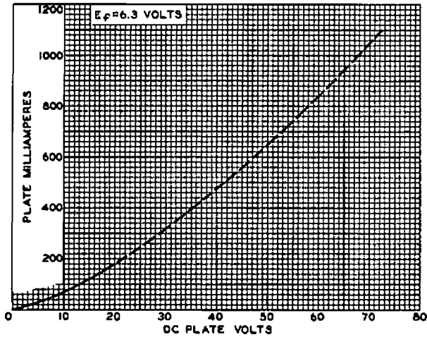
Fig. 1 - Average Plate Characteristic for Type 6AY3 and for Types 12AY3 and 17AY3 Except for Heater Voltage.
